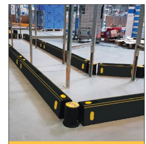
Corner post protection for increased deflection at areas typically susceptible to collision such as corners and angles, whilst enabling multi-directional kerb configurations.
